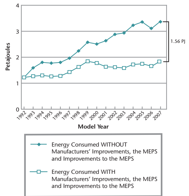
Figure 4 Annual Energy Savings for Refrigerators, 1992–2007
